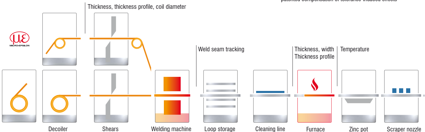
Additional measurement of width and cambering with patented compensation of tolerance-induced effects
